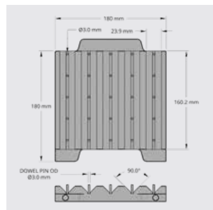
Prismenplatte 5-groove fixture tray
