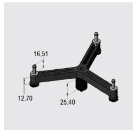
Spider Klemme SC 152 Spider clamp SC 152
